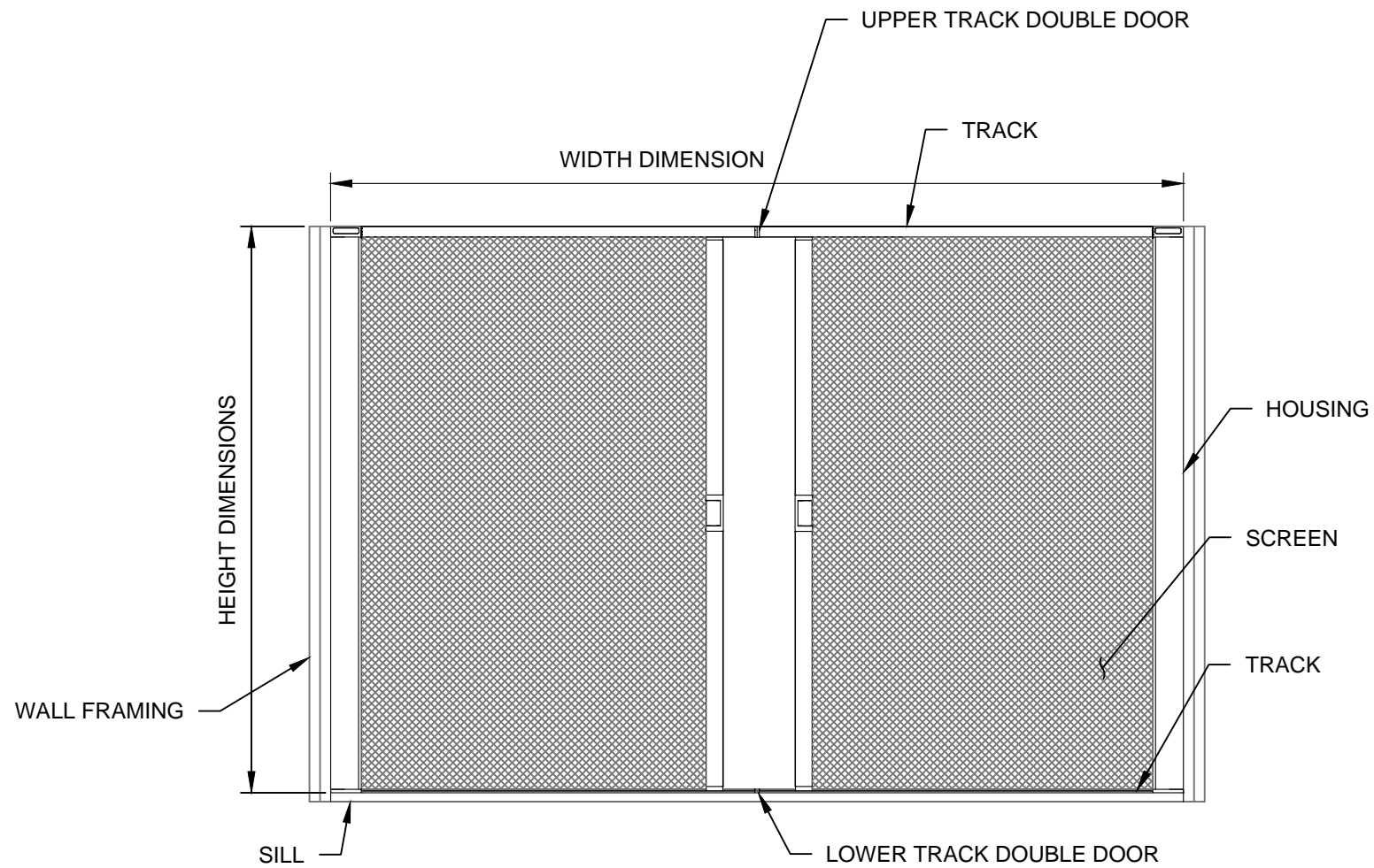
HORIZON DOUBLE DOOR TYPICAL ELEVATION
