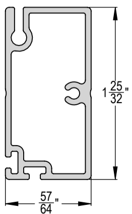
SIDE VIEW OF PULL BAR
