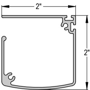
SIDE VIEW OF HOUSING
