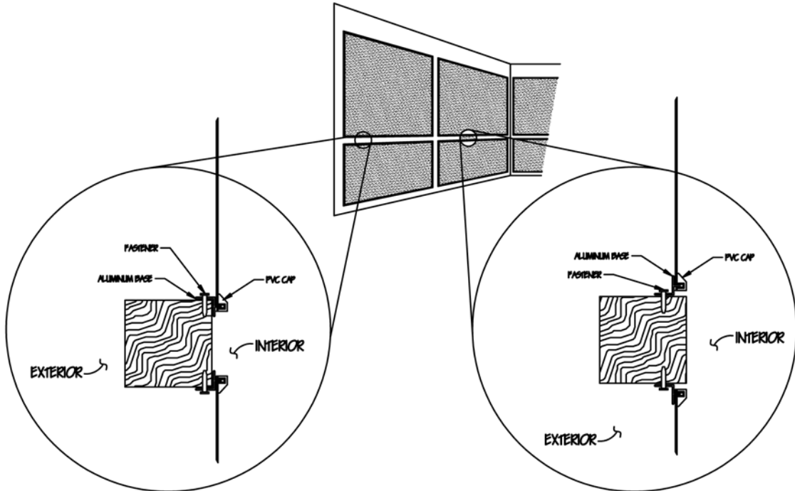
FLUSH MOUNT DETAIL SEE FRAMING DETAILS FOR FURTHER INFORMATION
